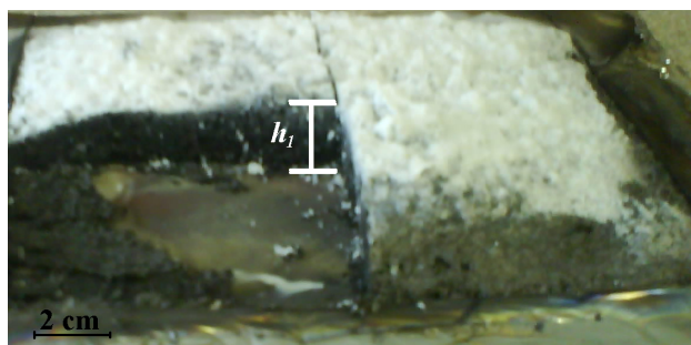
Fig. 7. Results of the fire protective coatings one-side heating tests
